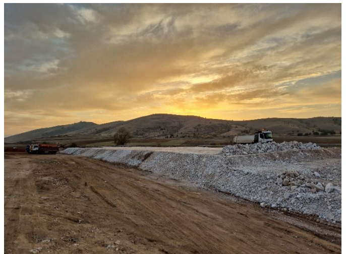
Photo 4: Section 4 Earthworks Operations
